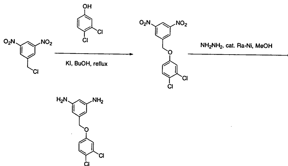
Scheme II-E
